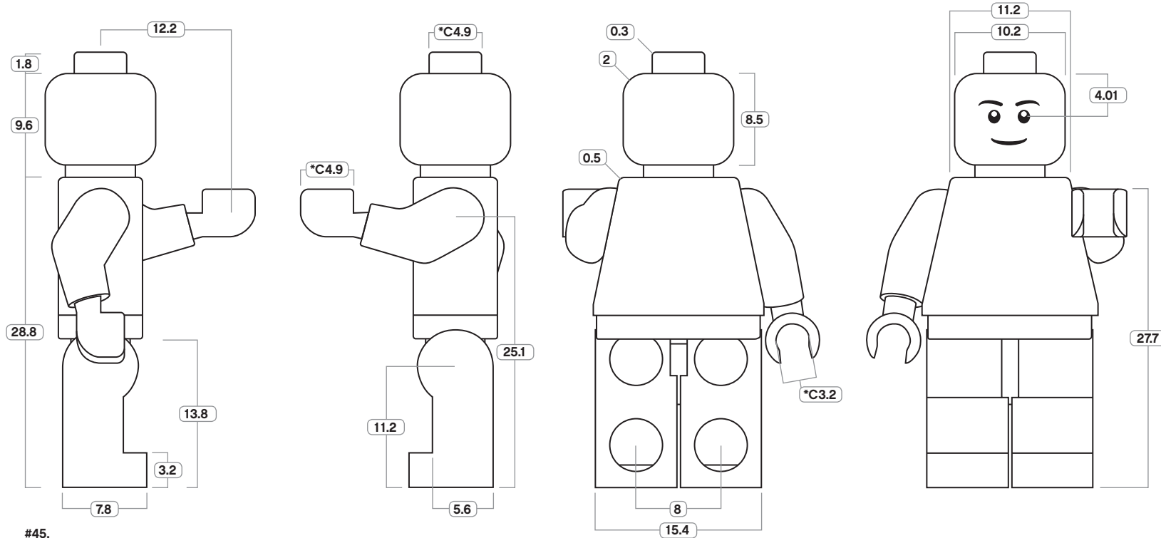
#45. Proportions of the LEGO® minifigure (in millimetres). Illustration in 2:1 and measurements in 1:1. *C: Circumference
